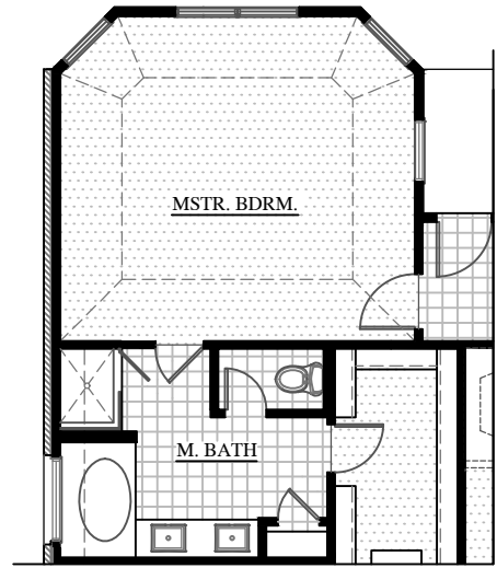
PARTIAL FIRST FLOOR PLAN - BAY WINDOW OPTION
