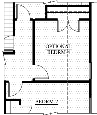
PARTIAL FIRST FLOOR PLAN OPT. BEDROOM 4
