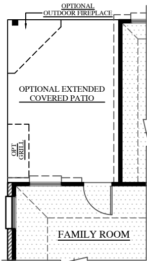
PARTIAL FIRST FLOOR PLAN OPT. EXT. COVERED PATIO
